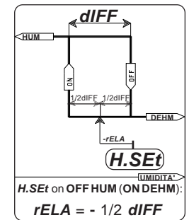
Swinging Ambient / Set humidity indicator
